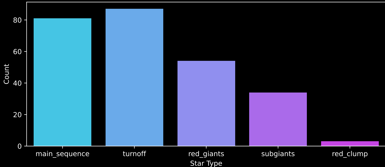
GALAH DR4 Field: [3009] Count plot of Star Type
