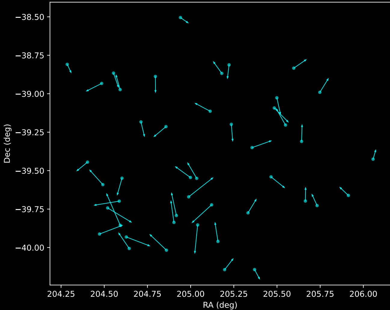
GALAH DR4 Noise Stream Proper Motion Vectors (n=45)
