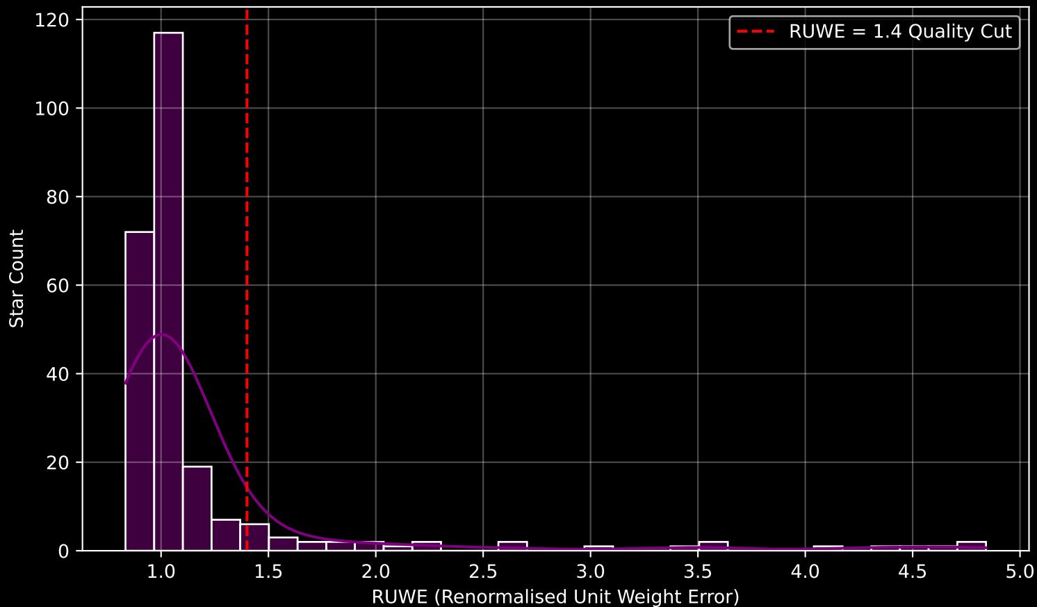
GALAH DR4 Field [3009] RUWE Distribution (n= 245)
