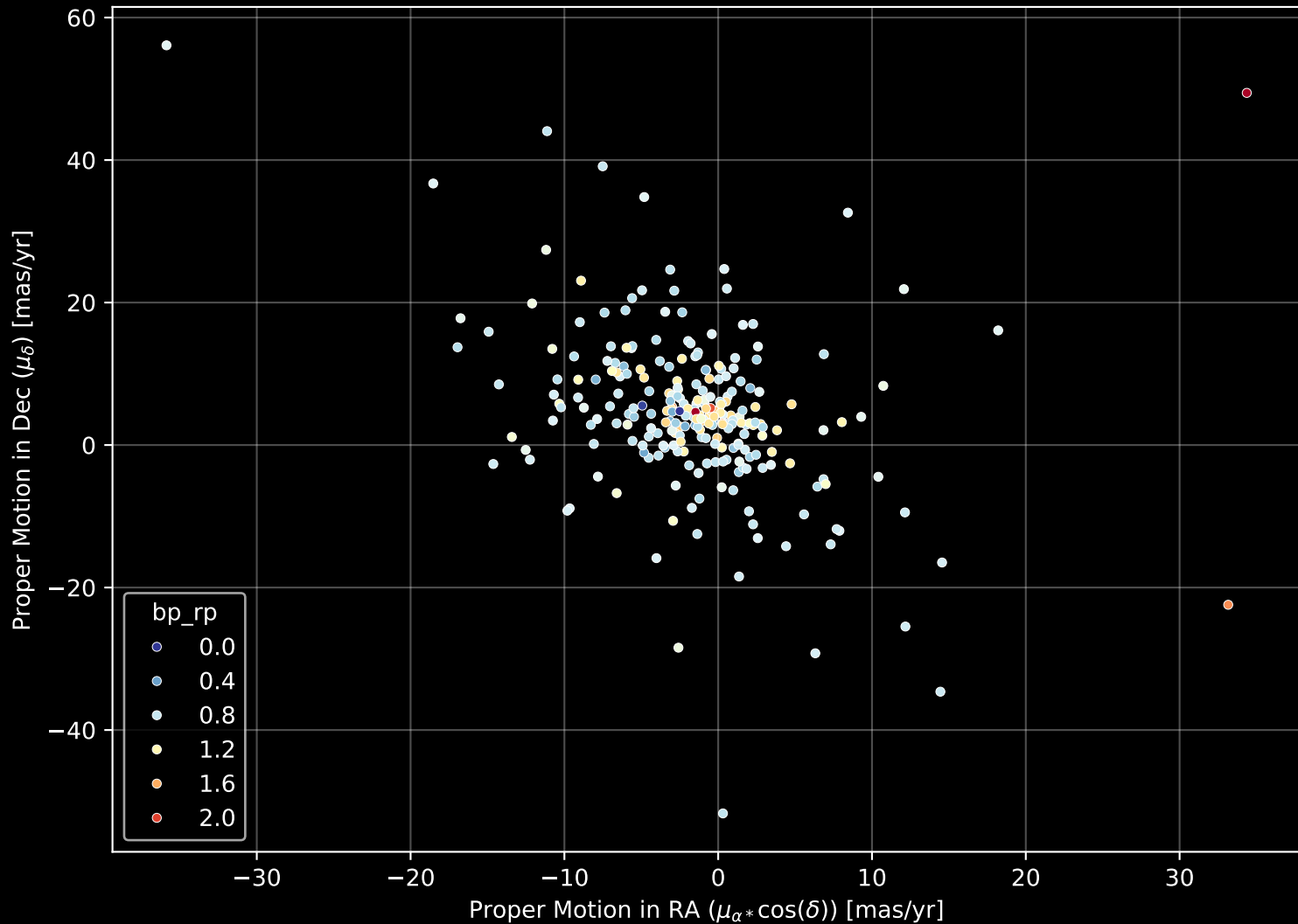
GALAH DR4 Field: [3009] Proper Motion Diagram (n= 259)
